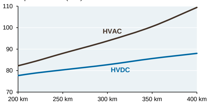
Transmission losses: HVAC vs HVDC
