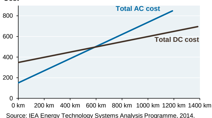
Comparison of HVAC and HVDC lifetime system costs
