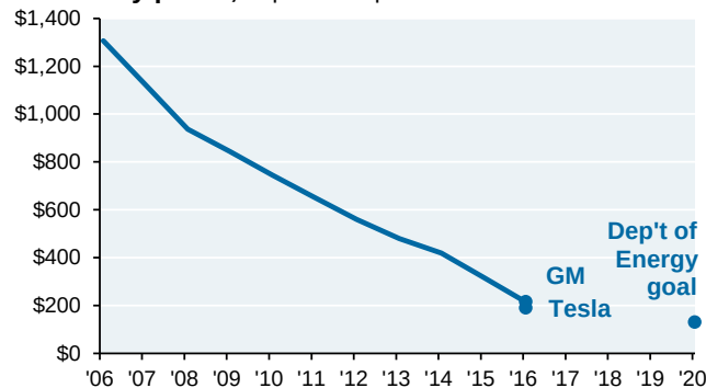
Lithium ion energy storage costs: EV battery packs, capital cost per kWh
