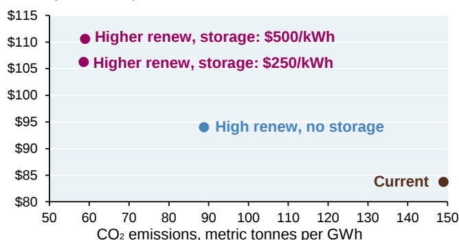
California electricity cost-emission tradeoffs, US$ system cost per MWh
