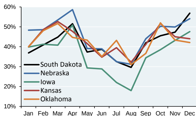
Wind capacity factors by month for Midwestern states
