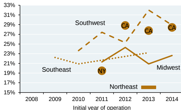
Solar capacity factors based on initial year of operation
