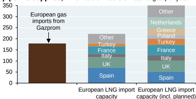
Europe LNG regasification (import) capacity vs Russian pipeline supplies , Billion cubic meters of natural gas per year
