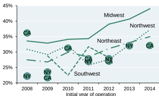
Wind capacity factors based on initial year of operation
