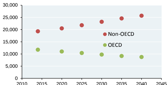
CO 2 emissions from OECD and non-OECD countries Million metric tonnes
