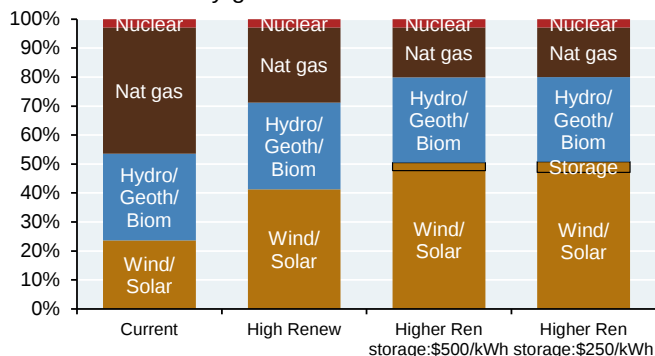
California electricity generation scenarios Share of electricity generation
