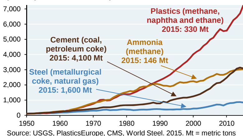
The 4 industrial pillars of modern society and their primary carbon-based inputs, Production index, 1950 = 100
