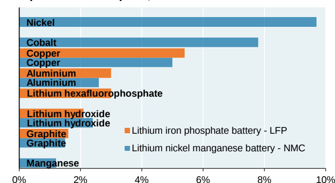
Change in battery prices assuming 100% increase in each component mineral price, Percent
