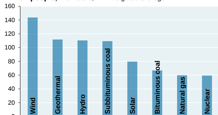
Distance required for power generation facilities to reach 2 million people, Kilometers, MW-weighted average
