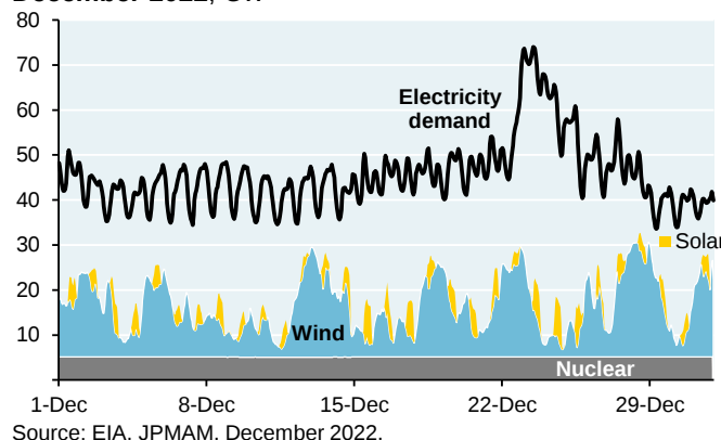
ERCOT baseload and renewable generation vs demand, December 2022, GW
