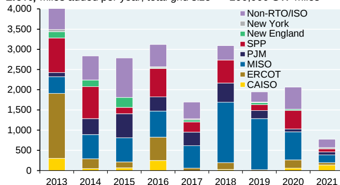
Recent transmission line growth has declined from 1.5% to 1.0%, Miles added per year, total grid size = ~200,000 GW-miles
