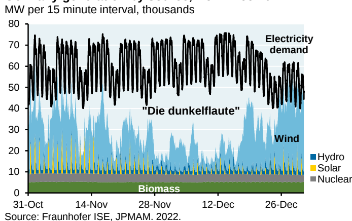
Germany generation by source, Nov - Dec 2022
